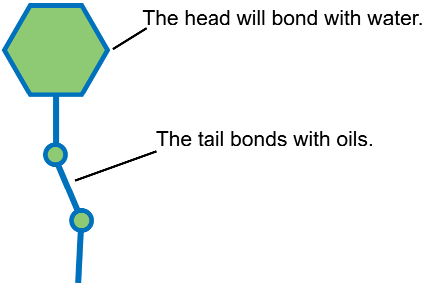
Soap Molecule
